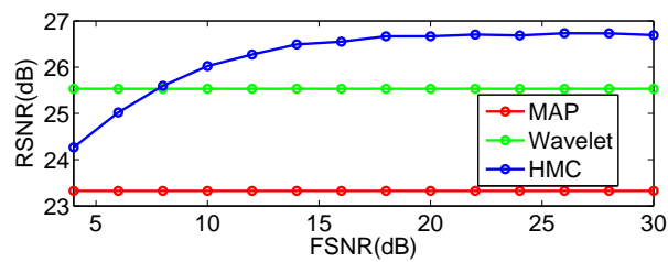
Fig. 6. Reconstruction errors of the different fusion methods versus FSNR.
