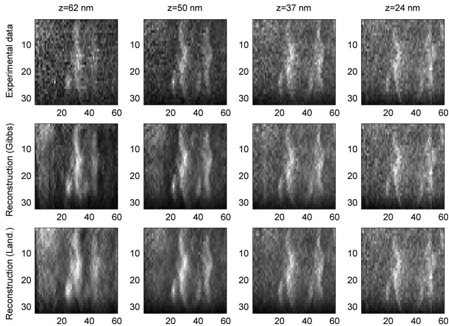
Fig. 12. Top: Experimental scan data where black (resp. white) pixel represents low (resp. high) density of spin (as in [8]). Middle: Scan data reconstructed from the proposed hierarchical Bayesian algorithm. Bottom: Scan data reconstructed from the Landweber algorithm.
